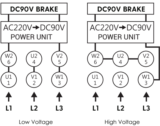
3 PHASE WITH 6 WIRES WITH BRAKE
