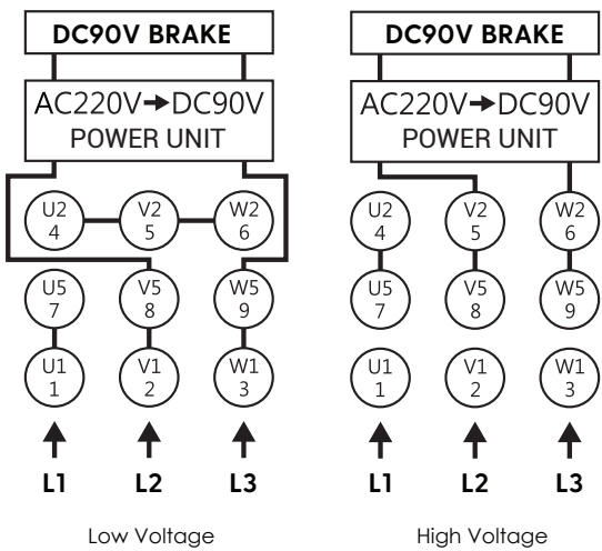
3 PHASE WITH 9 WIRES WITH BRAKE
