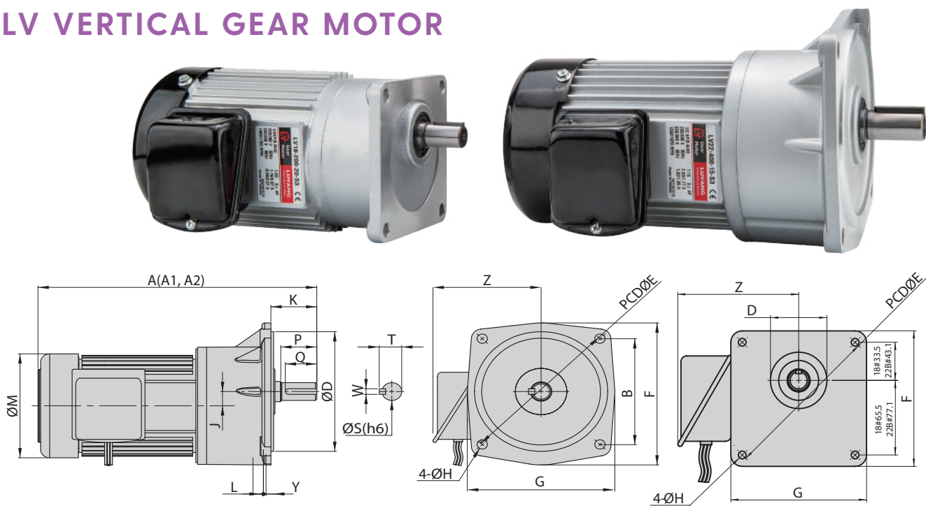
A FLANGE (For Code 22, 28, 32, 40, 50)
