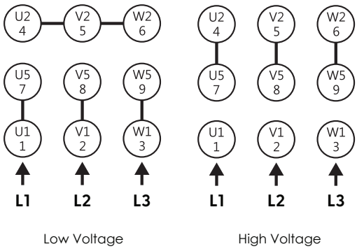
3 PHASE WITH 9 WIRES
