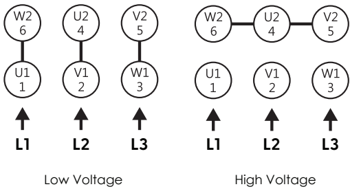
3 PHASE WITH 6 WIRES
