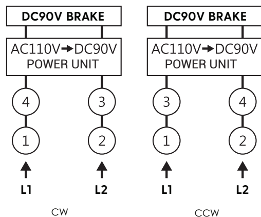
J SERIES-1 PHASE 110V WITH BRAKE
